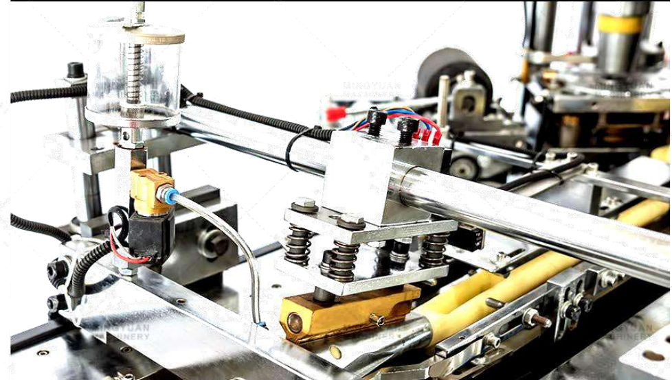
COPPER HEATER
